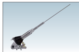
AH-2b ANTENNA ELEMENT A 2.5m long antenna element for mobile operation with the AH-4. All bands between 7–54 MHz can be matched.
